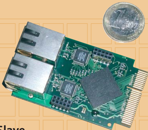
EtherCAT Interface with FPGA (IDAM)
