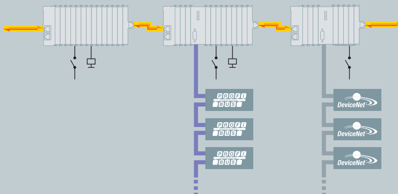
■ Figure 9: Decentralized Fieldbus Interfaces
