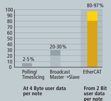
Figure 2: Comparison of Bandwidth Utilisation
