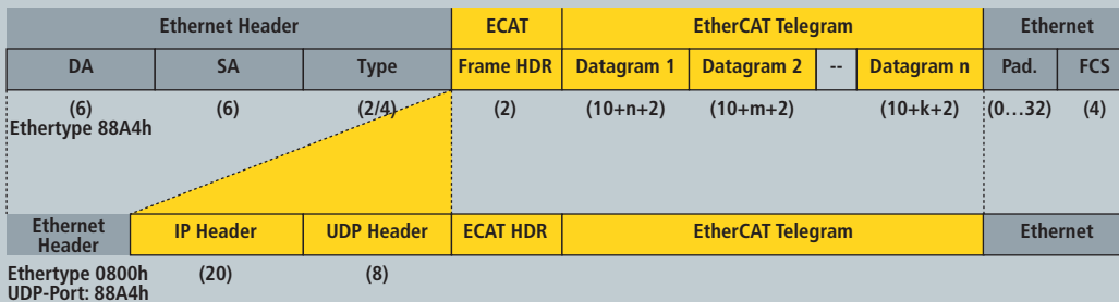
■ Figure 4: EtherCAT: Standard Frames according to IEEE 802.3 [3]
